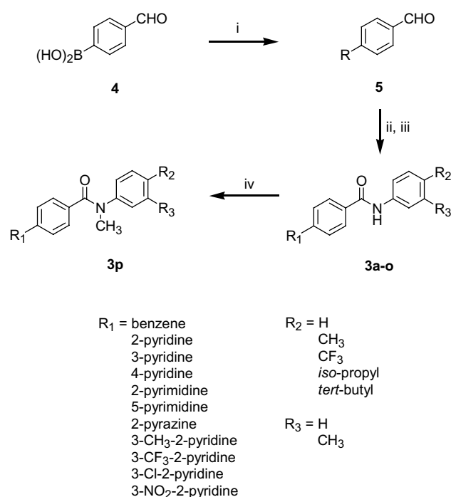
Scheme 1. Reagents and conditions: (a) (i) R 1 X, Pd(PPh 3 ) 4 , MeCN, 0.4 M NaHCO 3 , reflux, 5 h, 40–70%; (ii) NaClO 2 , NaH 2 PO 4 ·2H 2 O, CH 3 CH=C(CH 3 ) 2 , tert -BuOH, H 2 O, rt, 2 h, 80–90%; (iii) 4-R 2 PhNH 2 , EDC, DMAP, Et 3 N, CH 2 Cl 2 , rt, 2 h, 70–80%; (iv) CH 3 I, NaH, THF, 0 °C, 92%.
