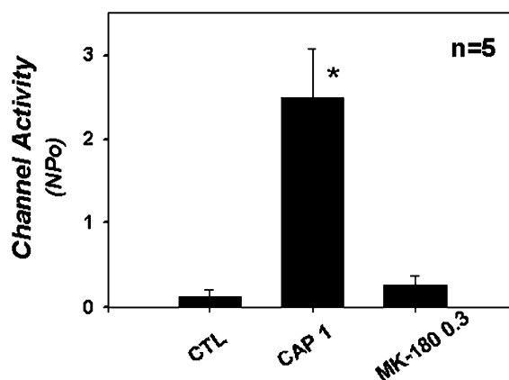
Figure 4. Comparison of the channel activity of capsaicin (1 \mu\text{M} ) to 2 (0.3 \mu\text{M} ) in the presence of capsaicin (1 \mu\text{M} ). CTL is control activity before the application of capsaicin.
