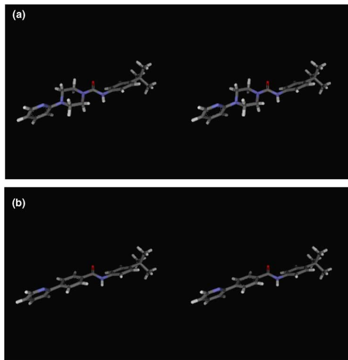
Figure 2. Stereoviews of the preferred three-dimensional conformations. (a) Energy-minimized conformation of 1 (5.113 kcal/mol); (b) energy-minimized conformation of 2 (6.786 kcal/mol).
