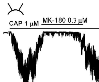
Figure 3. Reversible antagonistic effects of 2 (MK-180) on the capsaicin receptor.
